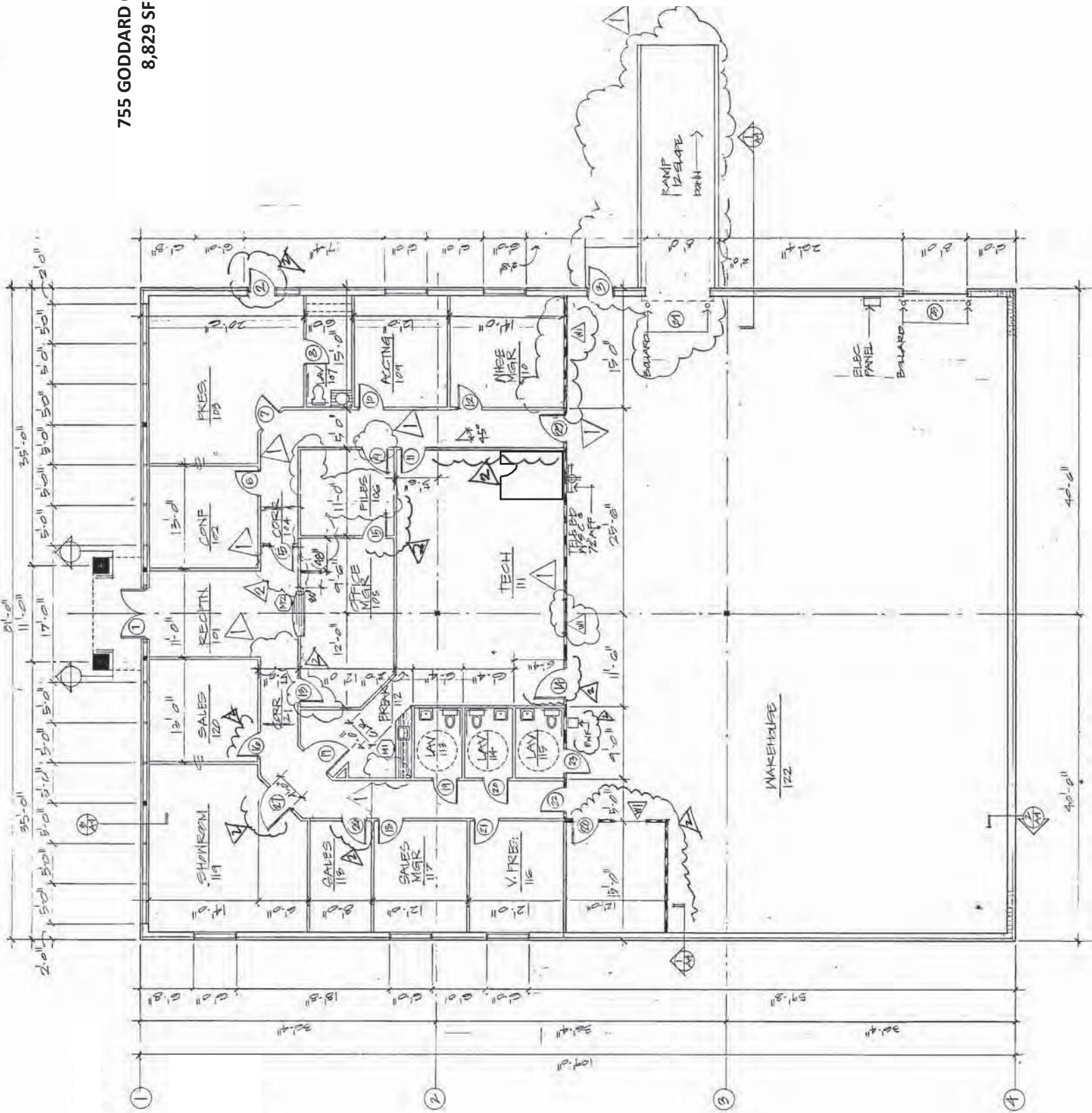
ARCHITECTURAL FLOOR PLAN
