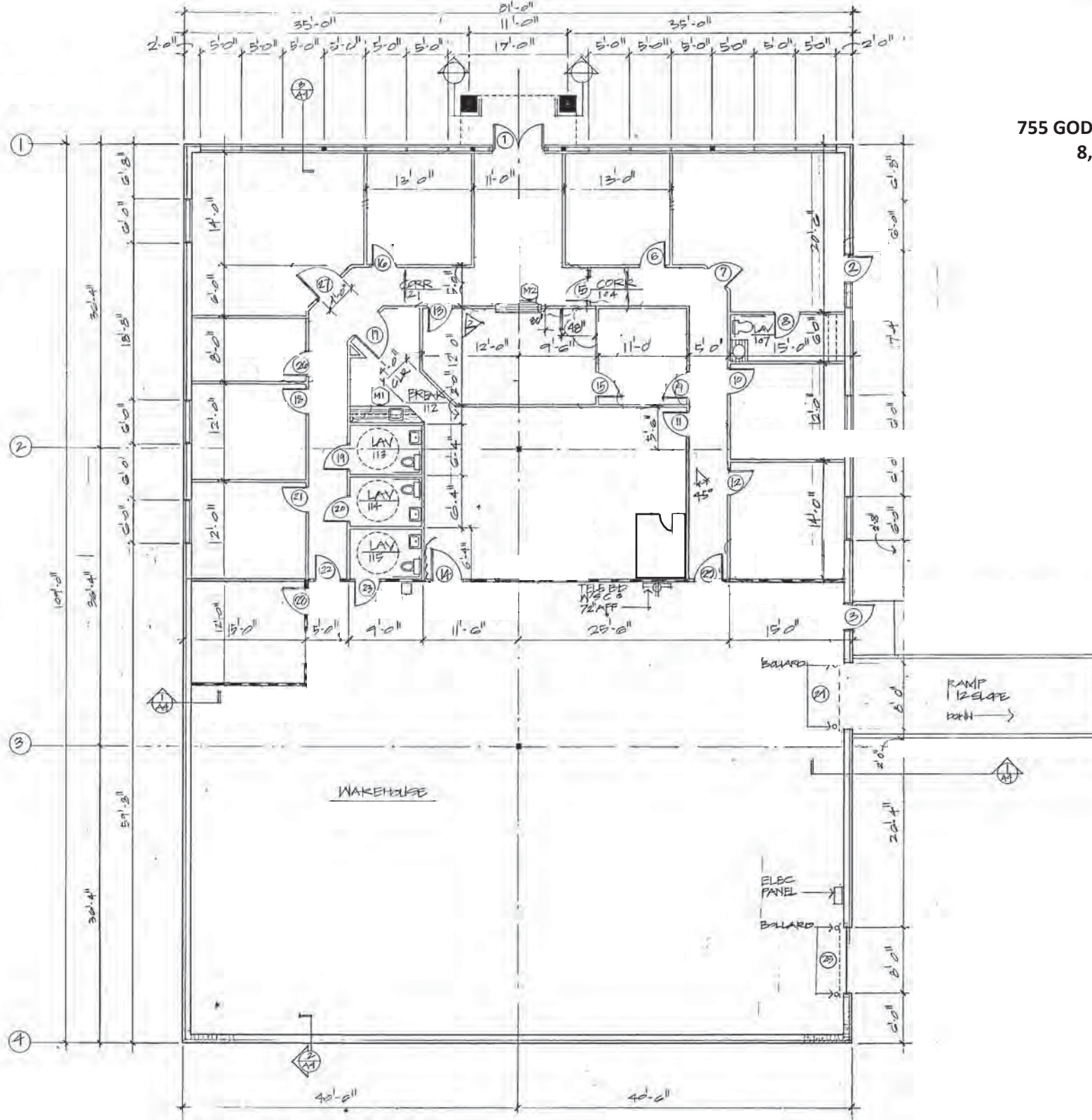
ARCHITECTURAL FLOOR PLAN
